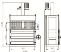
Diagram (Model XTY-500LE15076-15)
